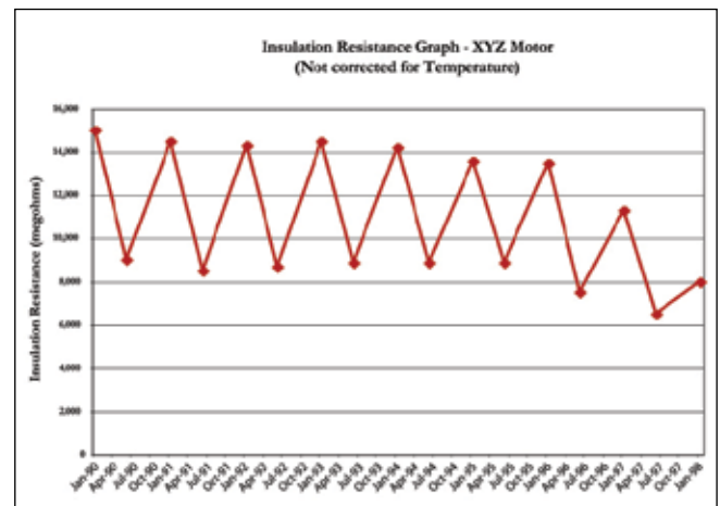
Figure 32: Insulation Resistance Graph Not Corrected for Temperature
