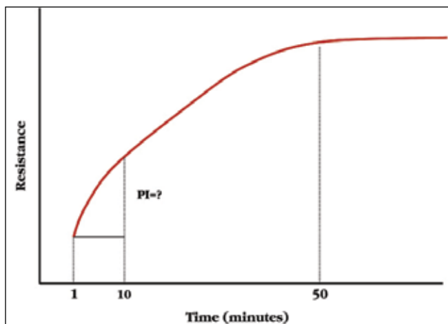
Figure 20: Benefit of the Polarization Test for Large Equipment
