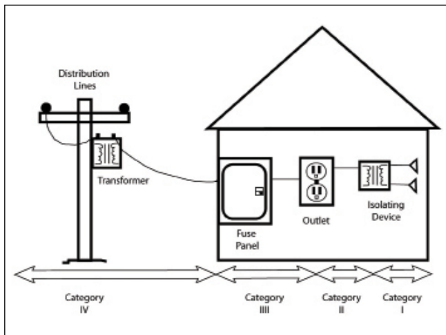
Figure 31: Electrical supply broken down into categories
