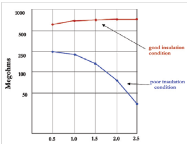
Figure 21: Step Voltage Graph
