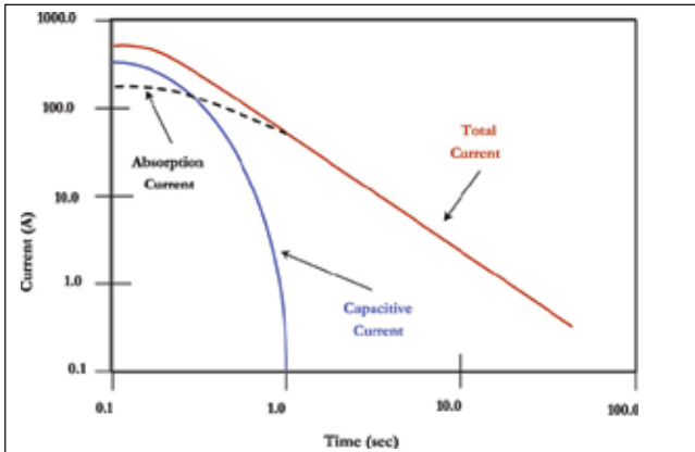
Figure 29: Reabsorption Currents
