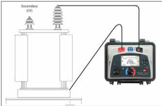
Figure 6: Connection to a Power Transformer
