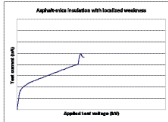
Figure 25: Asphalt-mica insulation with localized weakness
