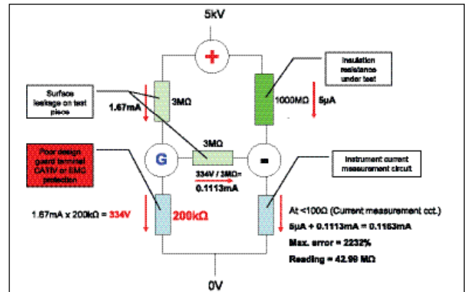
Figure 15: Measurement circuit "protected" by high impedance guard
