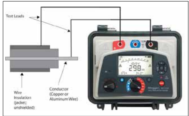
3: Simplistic Connection to a Cable
