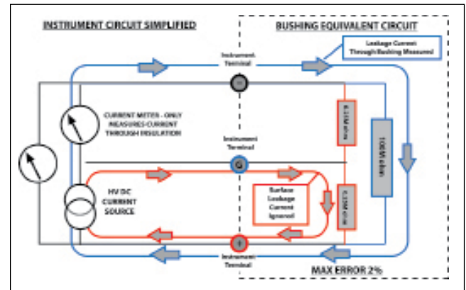
Figure 14: Instrument circuit simplified
