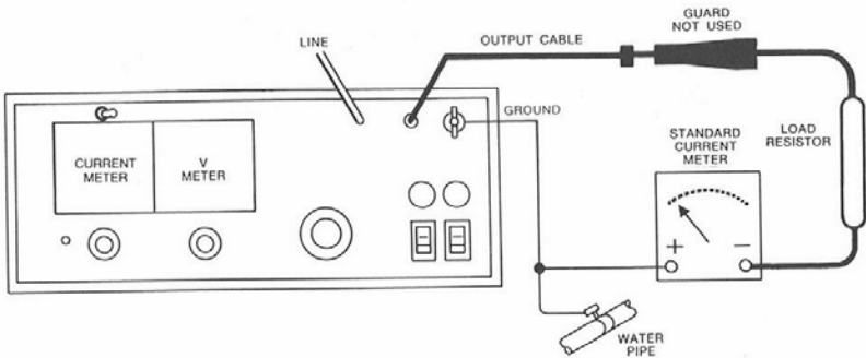
Figure 20: Connections for Calibration of the Current Meter
