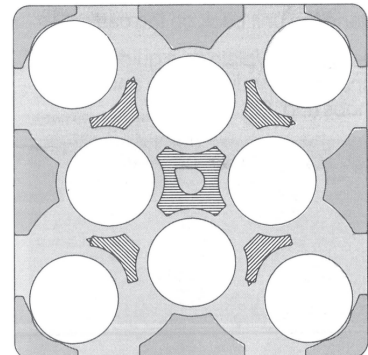
6½" TO 7¾" (165 to 185mm) DISH/PLATE DIAMETER 8 COLUMNS
