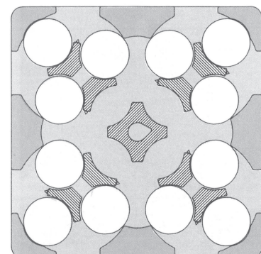
4¾" TO 5⅝" (120 to 135mm) DISH/PLATE DIAMETER 12 COLUMNS
