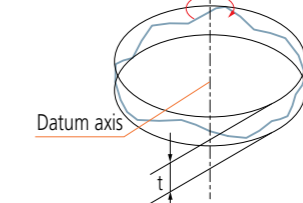
Verification example using a roundness measuring instrument
