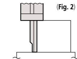
Scale Shift Error measurement example- depth measurement
