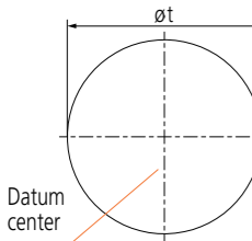
Verification example using a roundness measuring instrument
