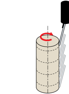
Verification example using a roundness measuring instrument
