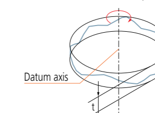
Verification example using a roundness measuring instrument
