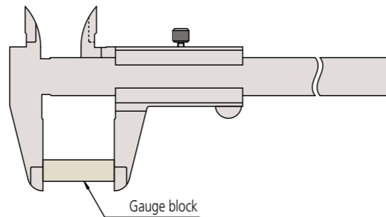
Fig. 3: Determining of partial measuring surface contact error
