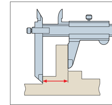
For stepped feature measurement
