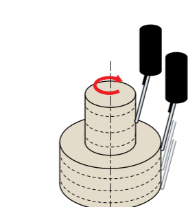
Verification example using a roundness measuring instrument
