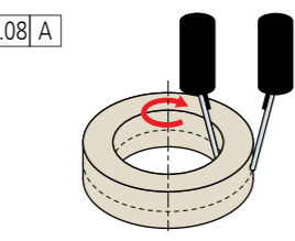
Verification example using a roundness measuring instrument
