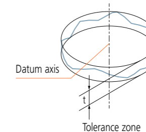
Verification example using a roundness measuring instrument
