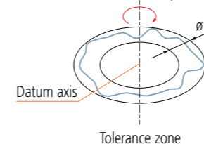
Verification example using a roundness measuring instrument
