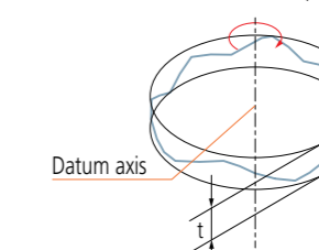
Verification example using a roundness measuring instrument
