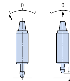
First contact. Plunger moves until the indicator reads zero.
