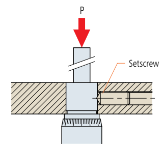
(3) Setscrew clamp
