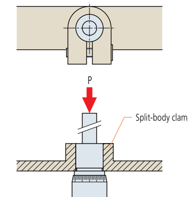
(2) Split-body clamp
