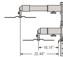
Ultra Short Throw Arm
