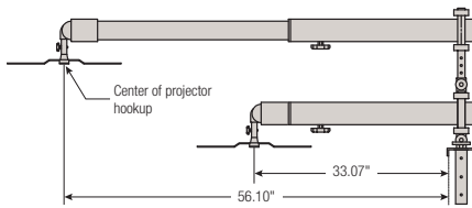
Short Throw Arm
