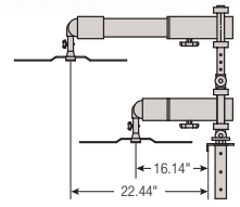
Ultra Short Throw Arm
