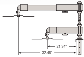
Super Short Throw Arm
