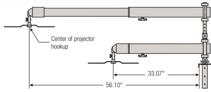
Short Throw Arm
