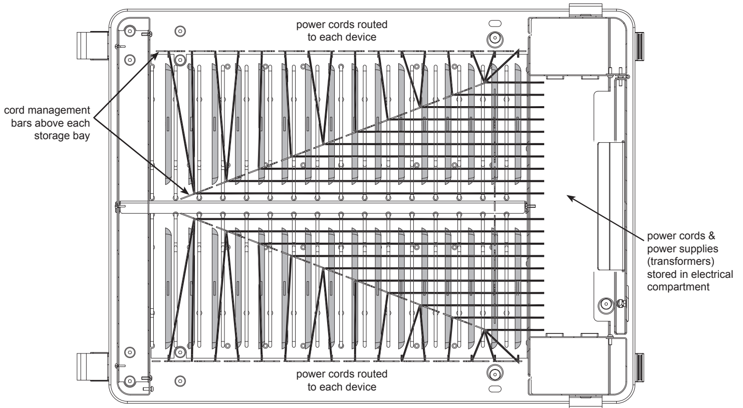
Top view of cord management bars and power cord routing from electrical compartment to computers
