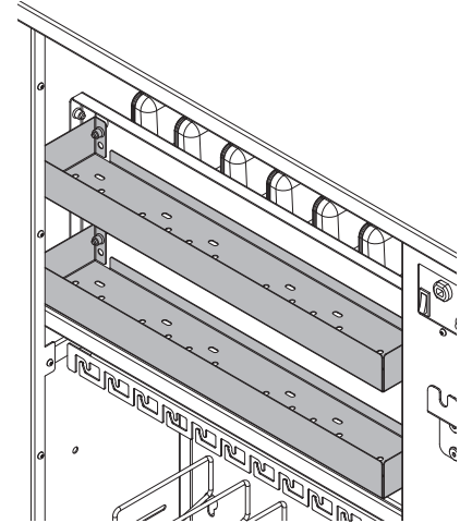
Power Supply Tray storage for cords, power supplies, or additional items 21 15 / 16 "W x 3 15 / 16 "D x 1 15 / 16 "H (max 2 per divider panel) 55487
