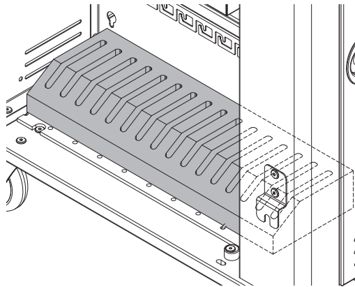
Small Device Foam Module stores smart phones & other small devices (16 slots) overall size: 23"W x 7 1 / 2 "D x 3"H slot size: 1/2"W x 5 1 / 2 "D x 1 5 / 16 "H 55486
