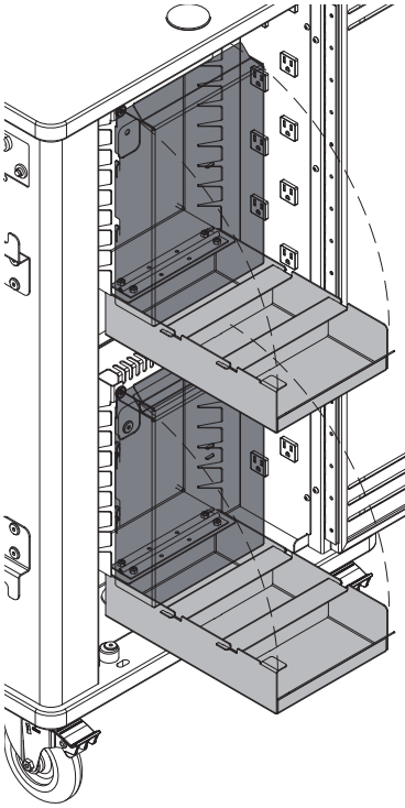
Power Cord Organizer (2 shown-max 2 per cart) 8"W x 5 1 / 16 "D x 13"H 55488
