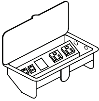
Power/Communication Module with 9' power cord, two outlets, two data jacks 7½"W x 3⅝"D 99003
