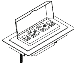
UL-Listed Power/Comm Module with 9' power cord, two outlets, two data jacks, & adapter plate 7½"W x 3⅝"D x ¾"H 99028
