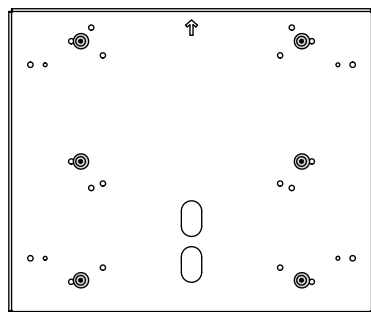
Mounting holes for NC1000C, NC1201L only
