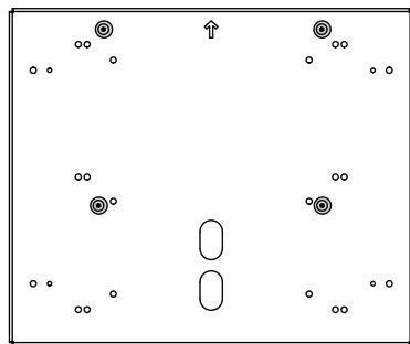
Mounting holes for NP-PA653UL (with NP44ML) NP-PA703UL (with NP44ML) NP-PA803UL (with NP44ML) only
