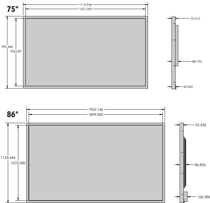
Dimensions shown in mm
