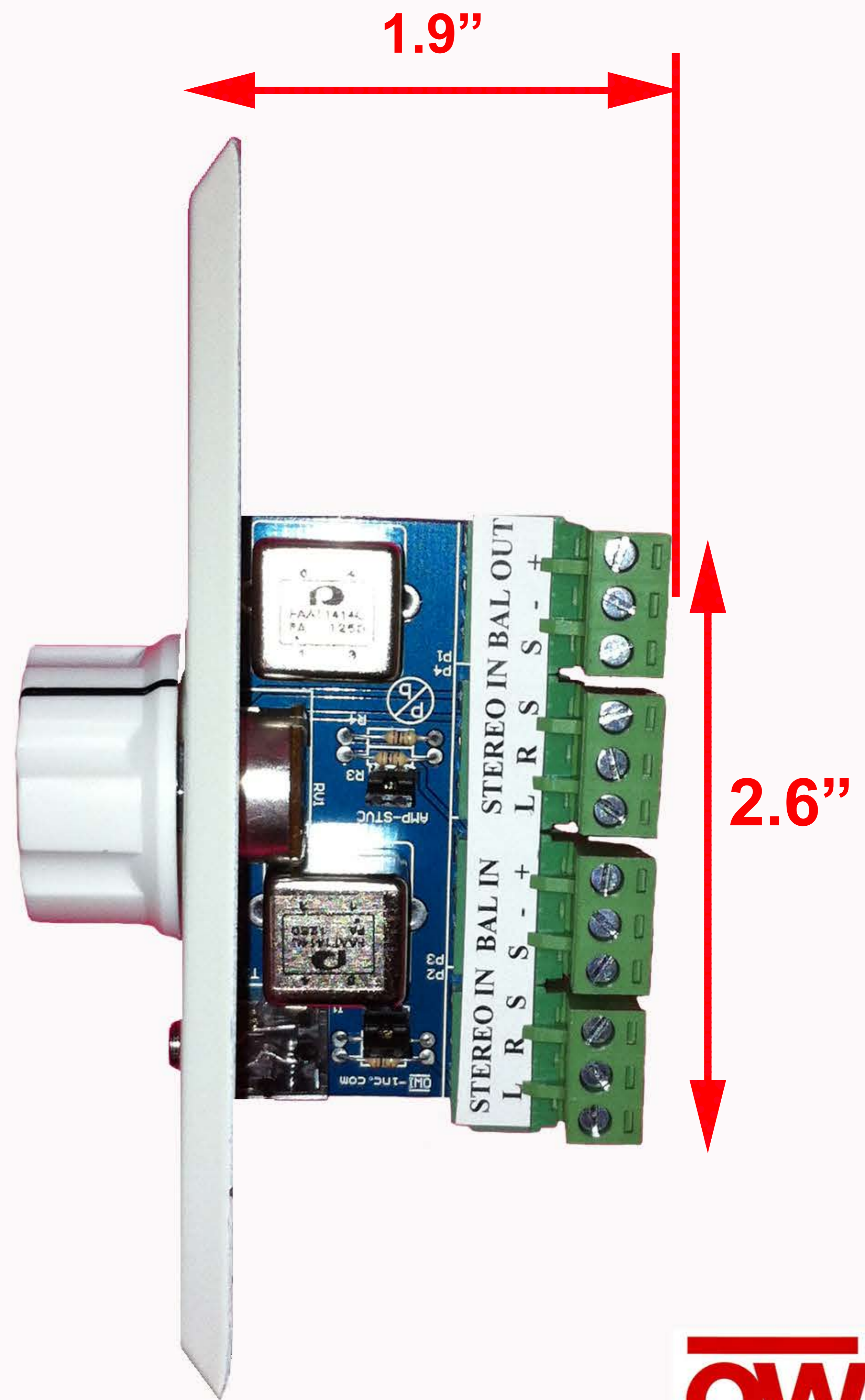
SIDE VIEW
