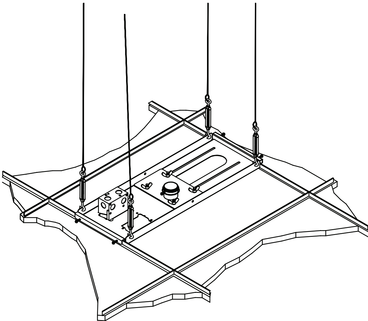
PP-FCTA Suspended Ceiling Adapter
