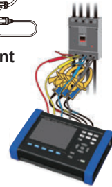
(Wiring image)
