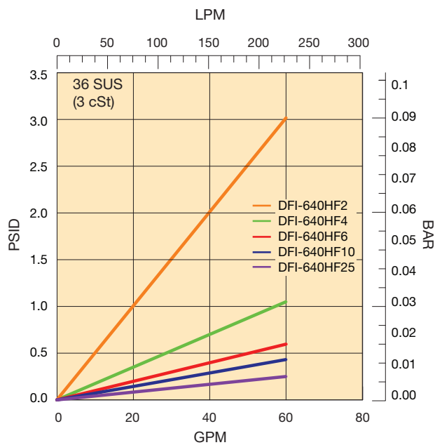
DFI-640... Flow vs Pressure Loss
