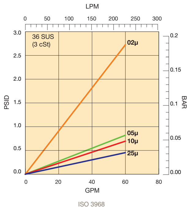
DFO-524... Flow vs Pressure Loss
