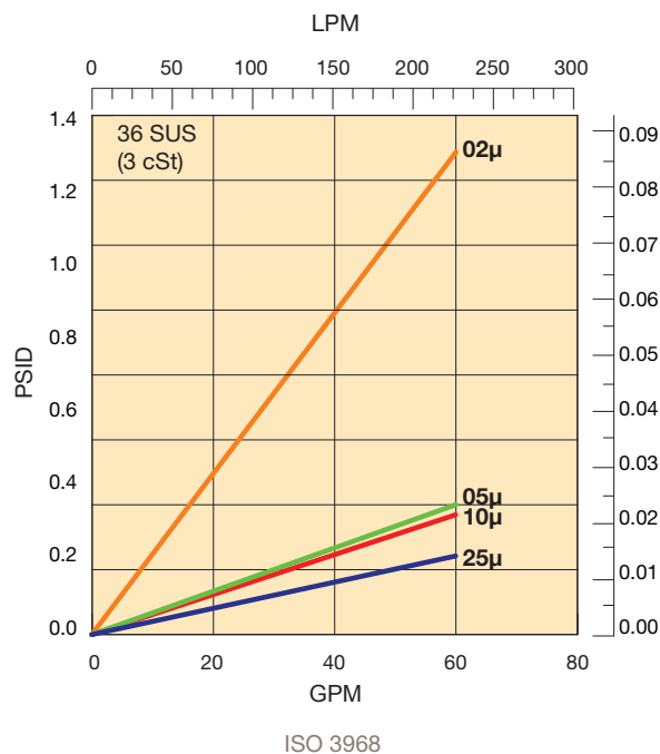
DFO-614... Flow vs Pressure Loss
