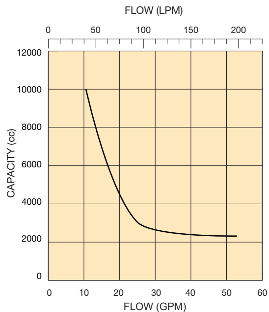
AD-52... Water Capacity
