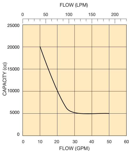
AD-65... Water Capacity
