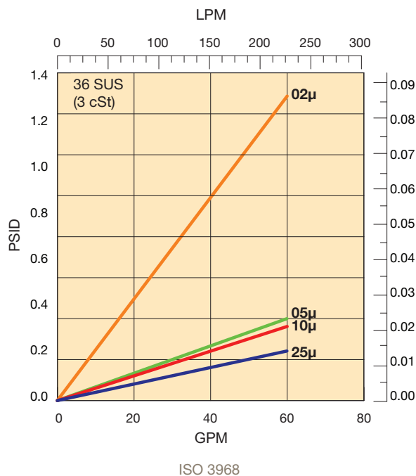
DFO-656... Flow vs Pressure Loss
