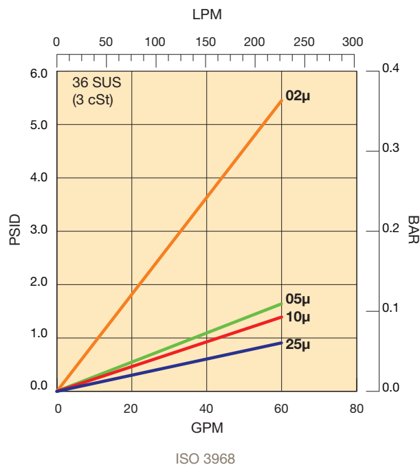
DFO-512... Flow vs Pressure Loss
