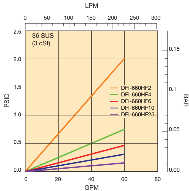
DFI-660... Flow vs Pressure Loss
