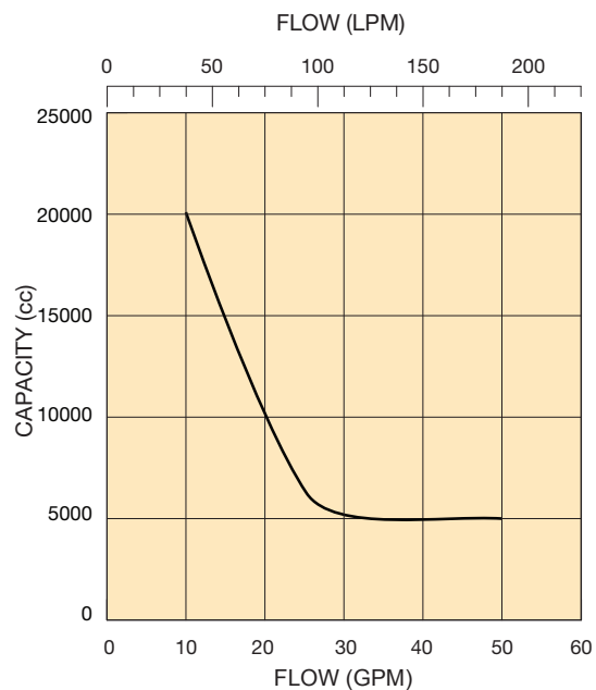
AD-61... Water Capacity
