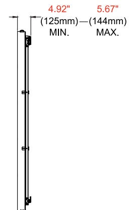
SIDE VIEW WITH MODULES
