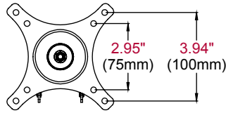
ADAPTOR PLATE
