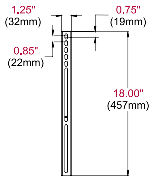
ADAPTOR BRACKET
