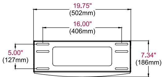
WALL PLATE
