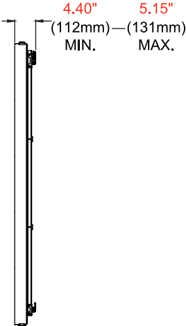
SIDE VIEW WITH MODULES
