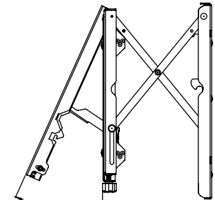
COMPONENT ACCESS
