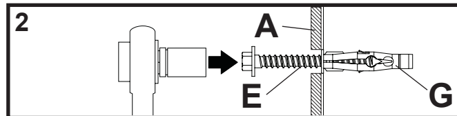
Place plate (A) over anchors (G) and secure with screws (E).
