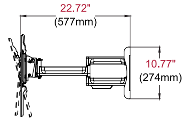
SIDE VIEW EXTENDED +15°/-5° TILT
