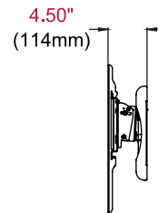
SIDE VIEW COLLAPSED
