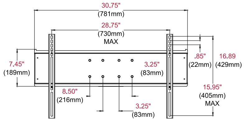
ADAPTOR DETAIL
