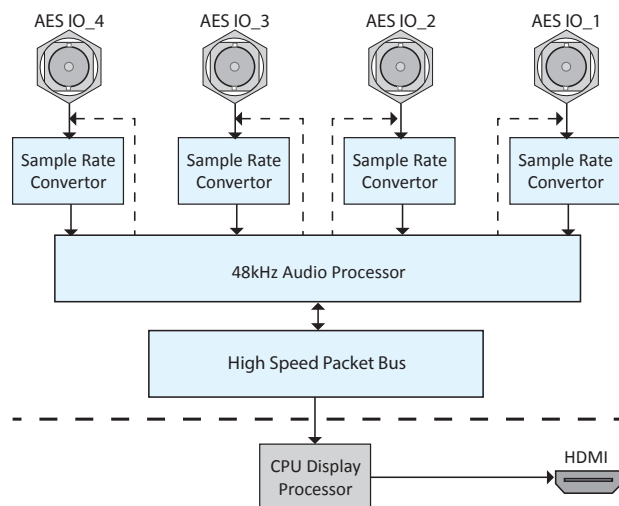
Schematic of the PHRXM-4AES module
