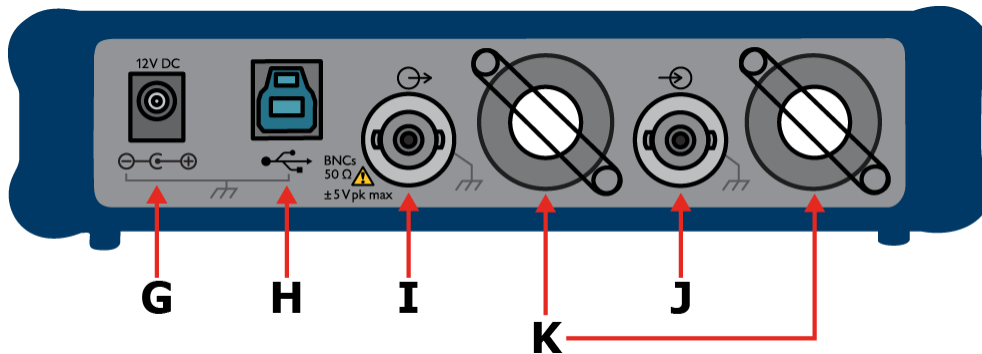
Rear panel: C and D models
