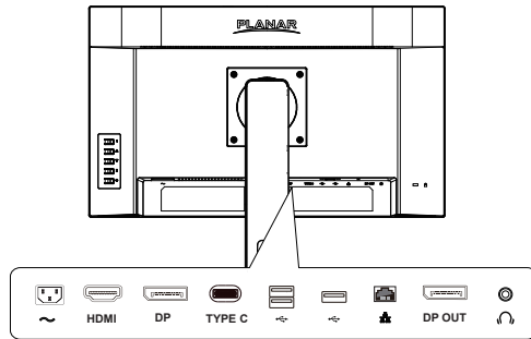
Figure 2 Connecting Cables
