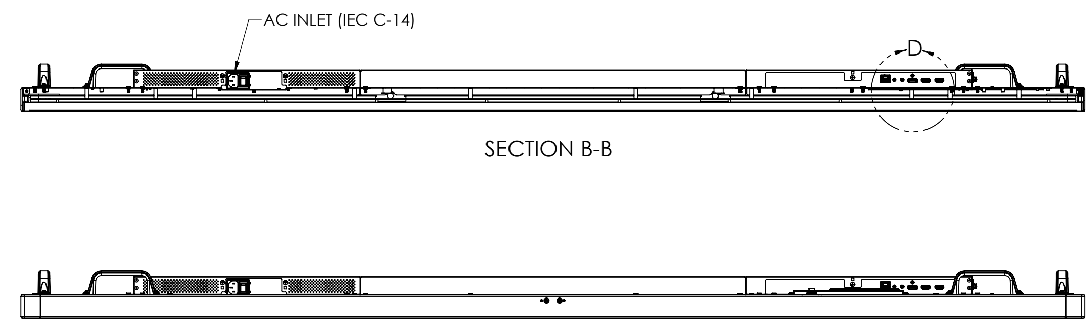
BOTTOM VIEW
