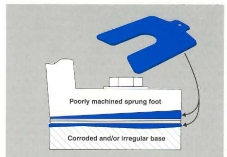
Sof' Shoe shims added to both sides of the shim pack "cold flow" to fill irregular gaps.
