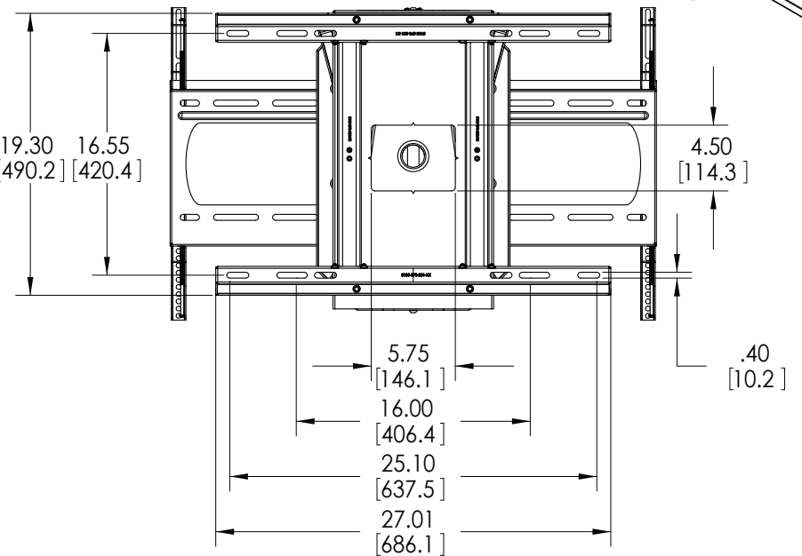
(FULLY COLLAPSED)
