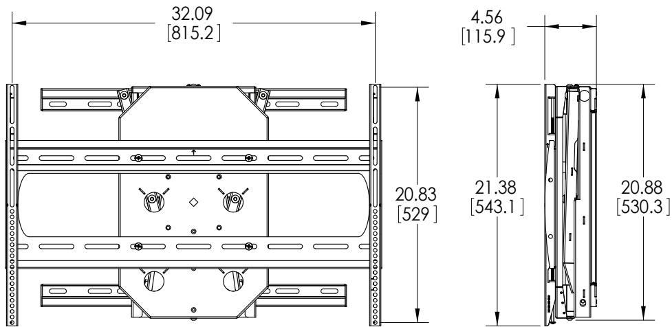
(FULLY COLLAPSED)
