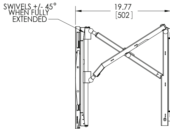
(FULLY EXTENDED)
