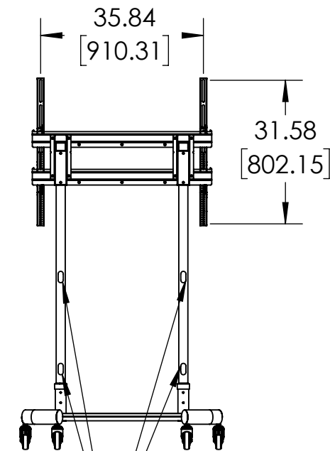
MAXIMUM VESA WITHOUT EXTENSION ADAPTERS
