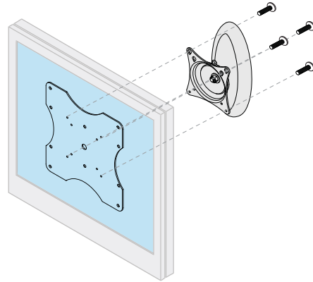
Flat Panel with UFP-280 Adapter Plate
