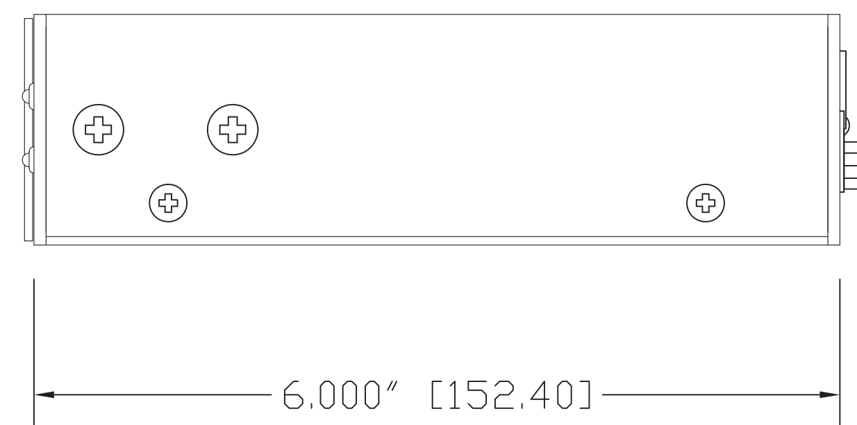
SIDE VIEW
