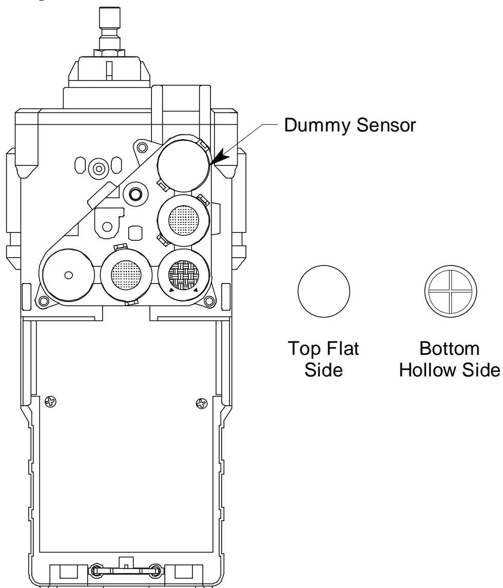
Figure 3: Dummy Sensor
