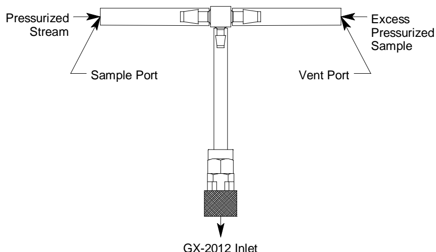
Figure 15: Purge Tee Fitting
