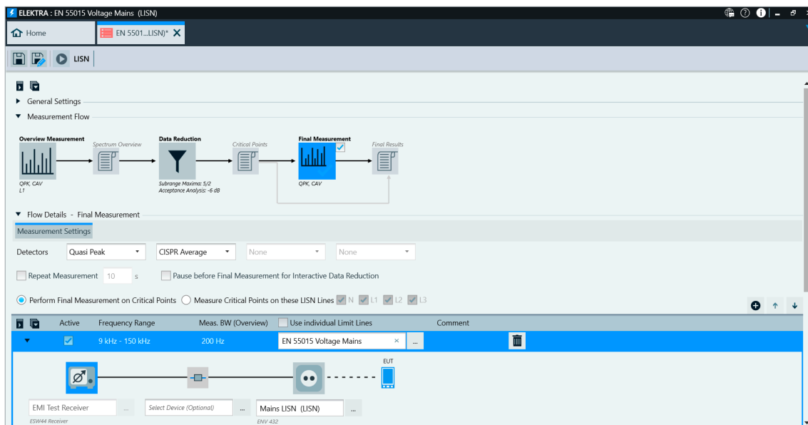
Test template for a conducted measurement with a LISN to measure a lamp (based on EN 55015 lighting equipment).
