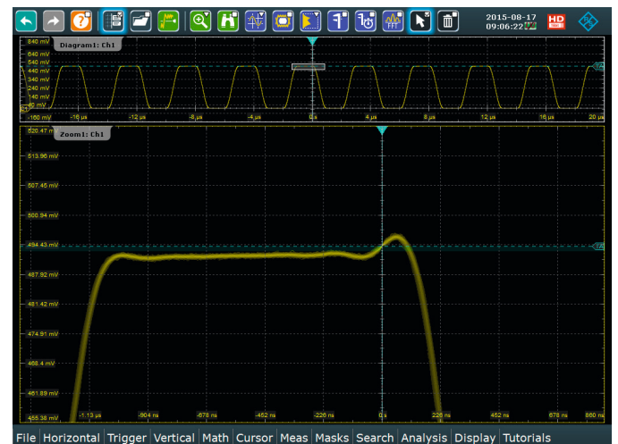
The unique architecture of the digital trigger permits stable triggering, even on signal details such as this 0.4% overshoot (high definition option).
