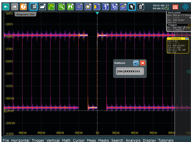
Serial pattern trigger set for a specific bit sequence with the R&S®RTO-K13 clock data recovery option.
