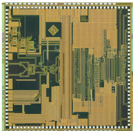
10 Gsample/s single-core A/D converter from Rohde & Schwarz.
