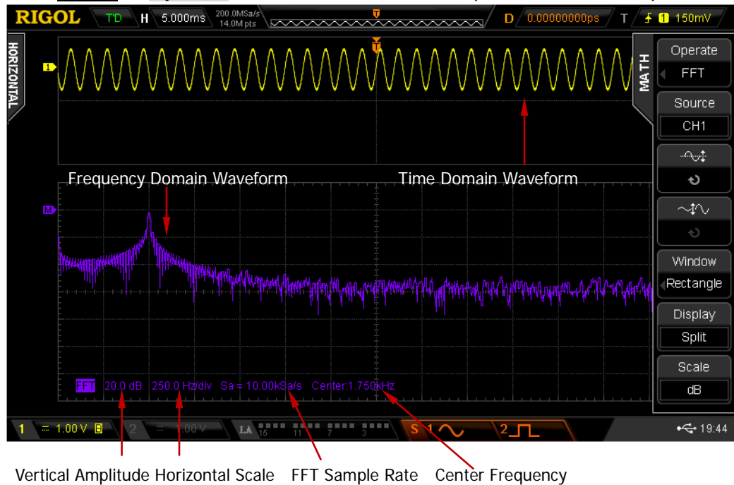
Figure 6-1 FFT Operation
