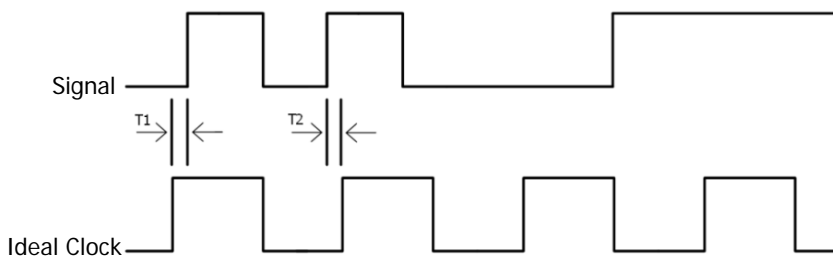
Figure 7-1 Digital Bus Jitter
