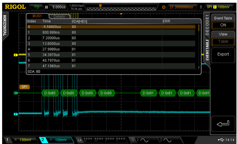
Figure 8-11 SPI Event Table
