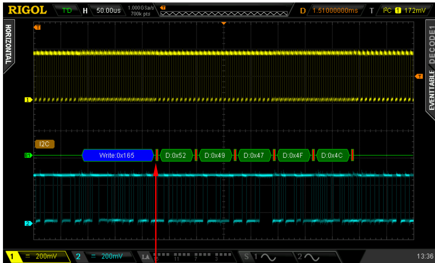
Figure 8-9 Error Expressions during Decoding
