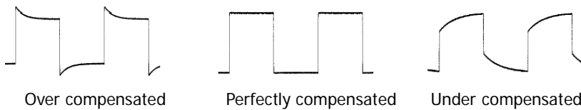
Figure 1-9 Probe Compensation
