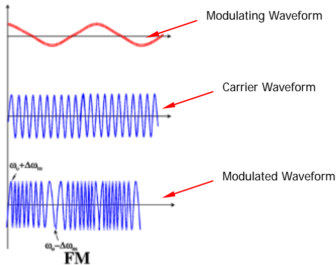
Figure 13-10 Frequency Modulation
