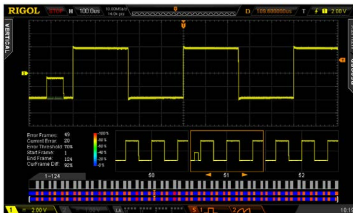
Figure 11-2 Analyze the waveform recorded
