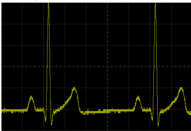
Figure 13-5 Analog ECG
