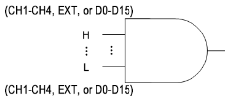
Figure 5-5 Pattern Trigger
