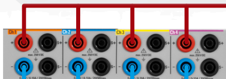
Parallel operation – max. 80 A
