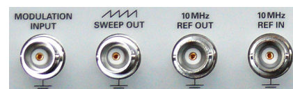
Fig. 7.3: Signal inputs and outputs including modulation input
