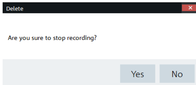
Figure 4-15: Delete dialog
