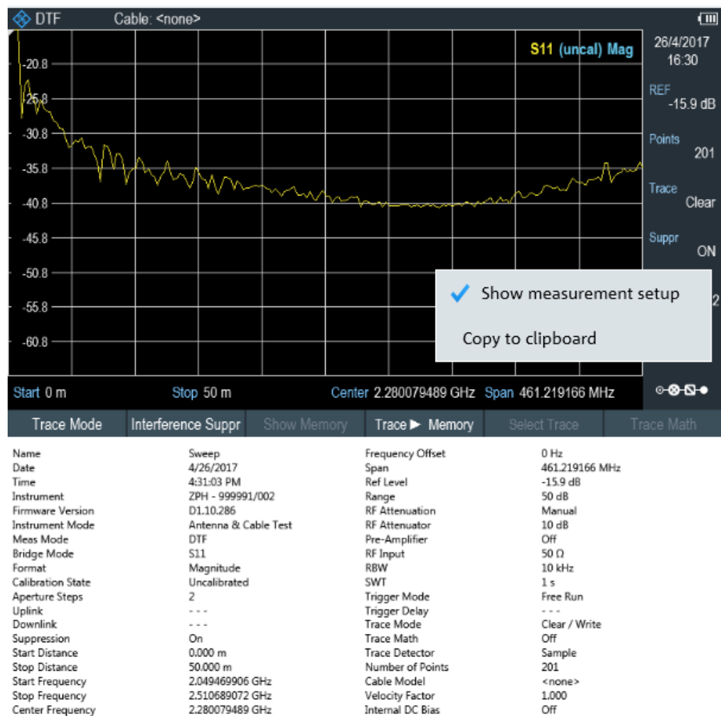
Figure 4-16: Screenshot
