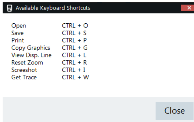
Figure 4-42: Shortcut keyboard
