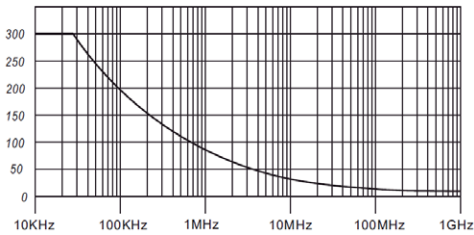
Fig. 1: Derating curve
