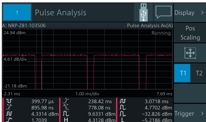
Automatic pulse analysis with the R&S®NRX and R&S®NRP-Z81
