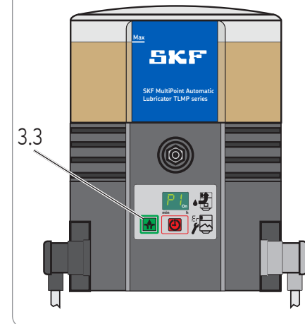
Trigger an additional lubrication Fig. 11
