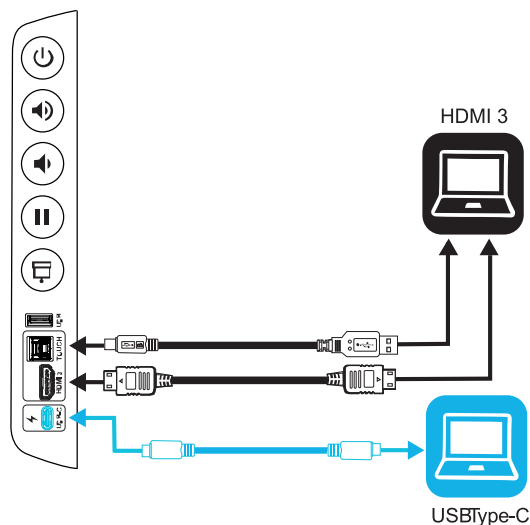
Convenience panel
