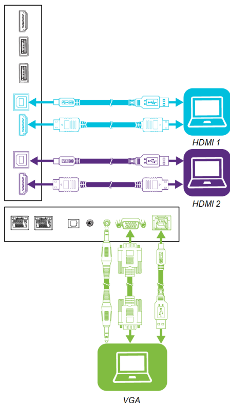
Connector panel
