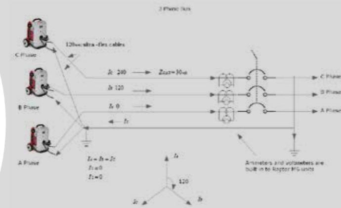
Figure 2: Test circuit for three phase primary current injection (4kV/10kV output)
