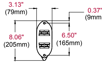
WALL PLATE
