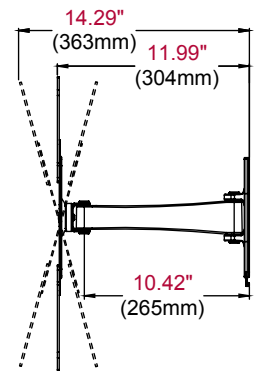
SIDE VIEW EXTENDED +/- 15° TILT
