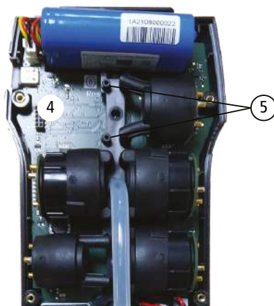
Sensor removed
