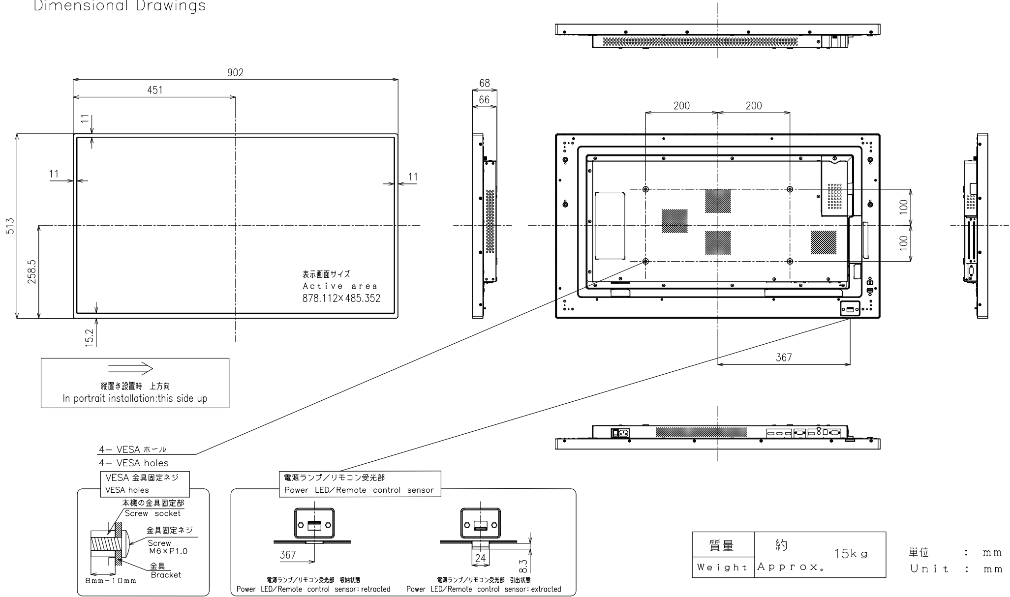
寸法図 Dimensional Drawings
