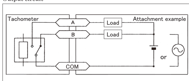
Output circuit
