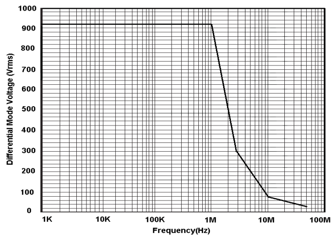
Figure 1: Max Differential Voltage versus Frequency Curve
